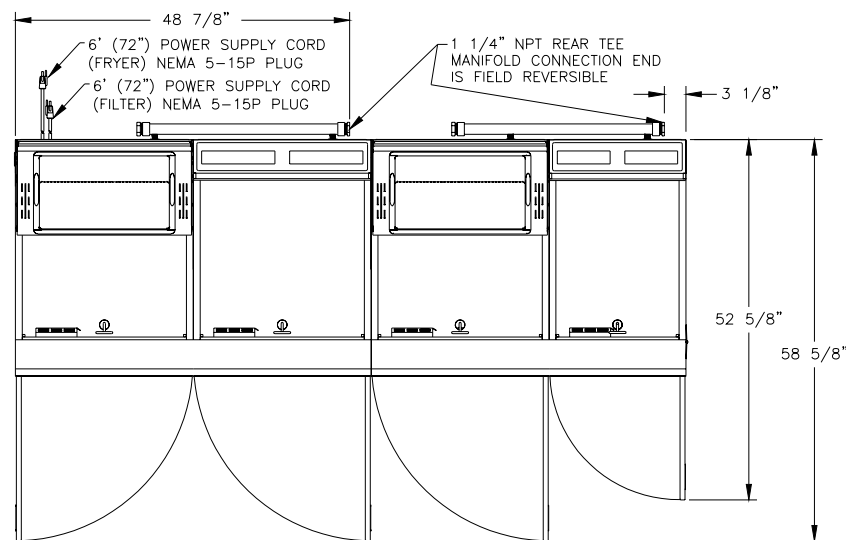
LJ-FBG24-3/FBG18 Fryers with Self Contained Oil Filtration System
