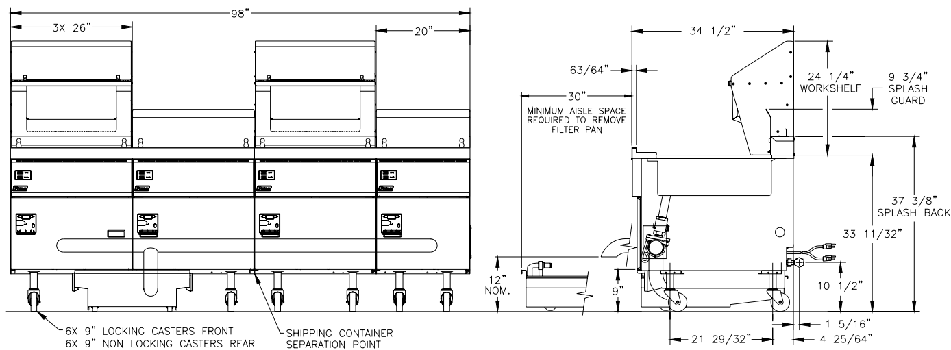
LJ-FBG24-3/FBG18 Fryers with Self Contained Oil Filtration System
